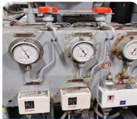
AC system
